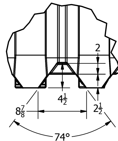
DETAIL A SCALE 1 / 11
