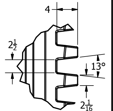
DETAIL C SCALE 1 / 11
