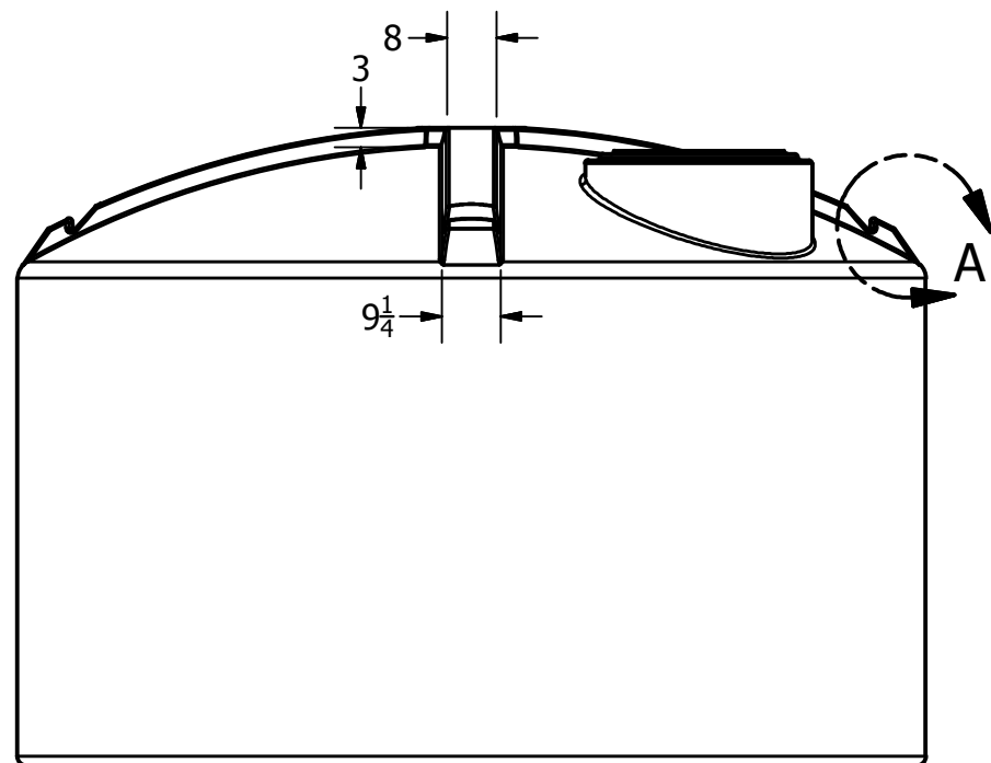
DETAIL A SCALE 0.06 : 1
