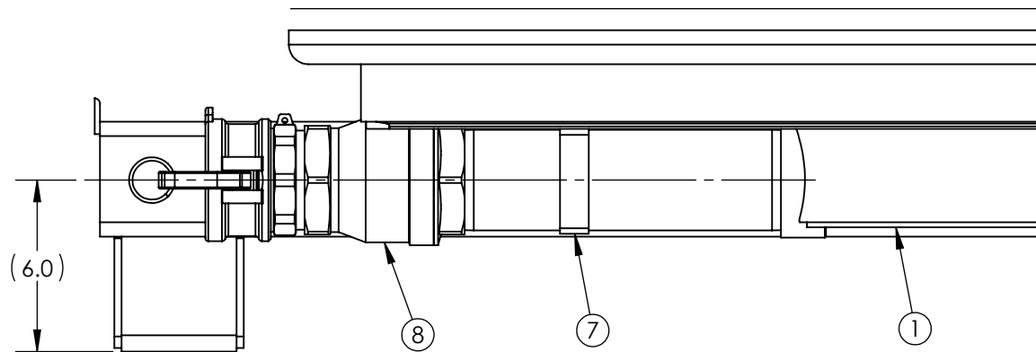
VALVE DETAIL
