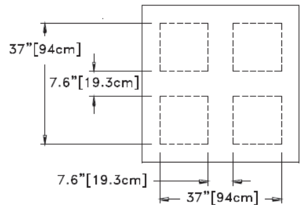
Optional Hand-Truck Bottom Cut-Outs
